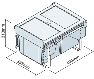
BIN38 Designed For Cabinets With Restricted Internal Height. Can Be Mounted To The Door Or Installed Behind A Standard Hinged Door. softCLOSE
