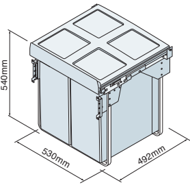
BIN39 Can Be Mounted To The Door Or Installed Behind A Standard Hinged Door. softCLOSE
